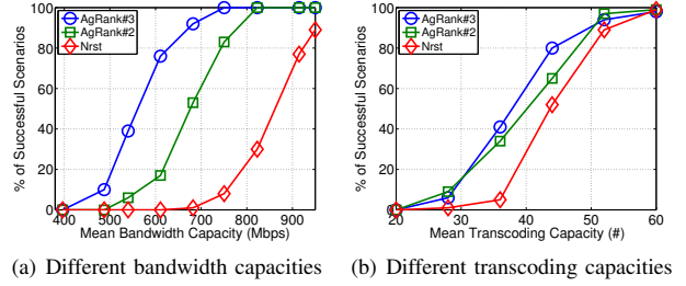
Fig. 9. Comparison of AgRank and Nrst
