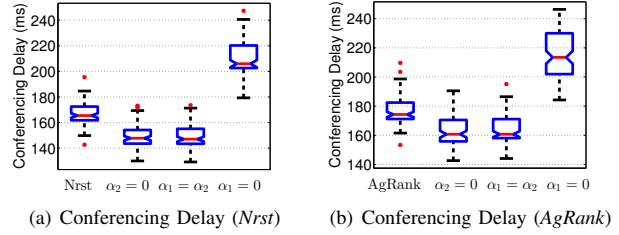
Fig. 8. Comparison of initial delay of AgRank and Nrst and the reduction by executing Alg. 1 with different design parameters
